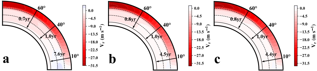
Figure 3. Inward velocity distributions. Three panels correspond to that of Figure 1 with the addition of inward pumping of Eq.(6). The black arrows indicate the transport time of the poloidal fields from the surface to the base of the CZ, at latitudes 10^\circ , 40^\circ , and 60^\circ .
